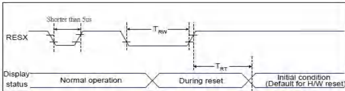
Figure 9 Reset Timing
